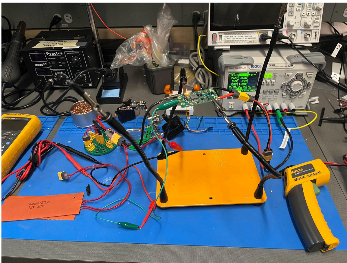
Figure 6.1: The test rig used for measuring regulation under load and thermal characteristics.
