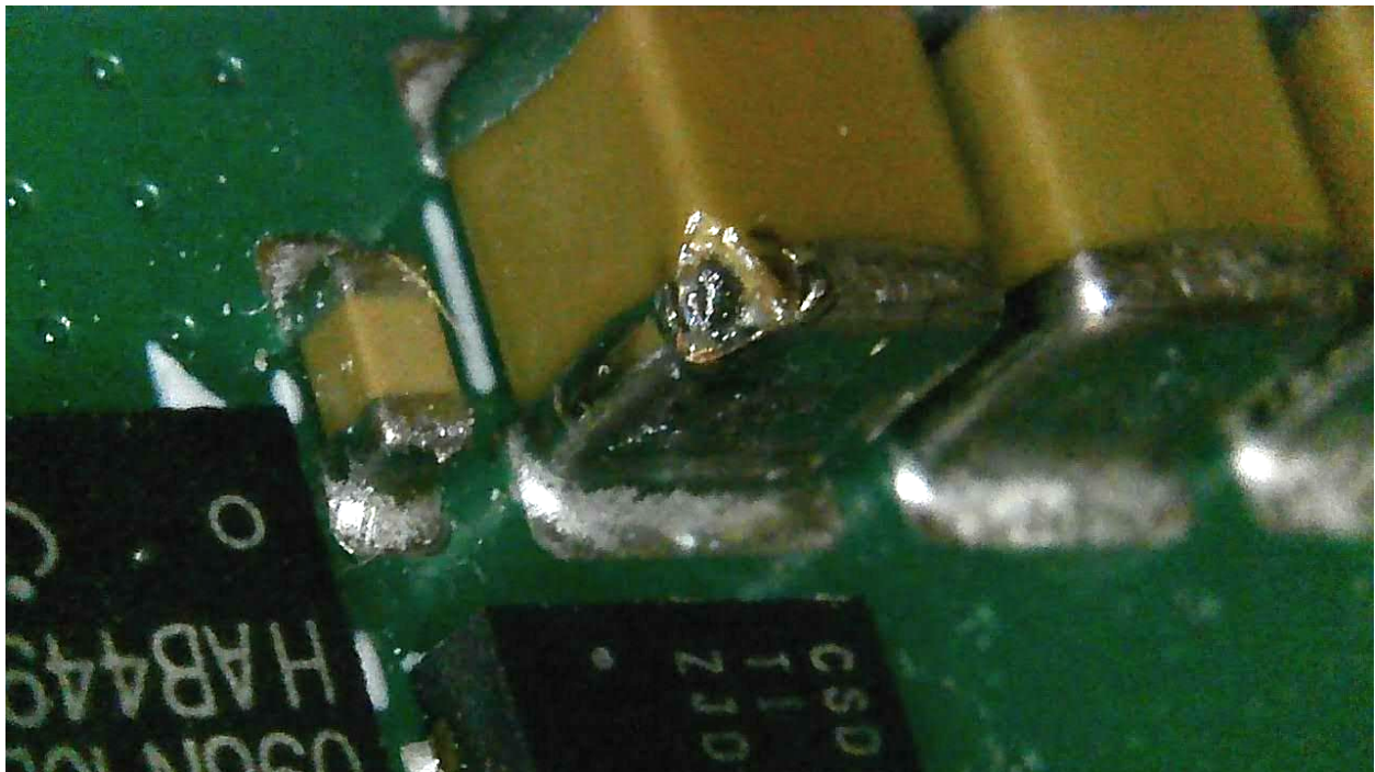
Figure 7.2: Microscope view of the damaged input capacitor from the side.
