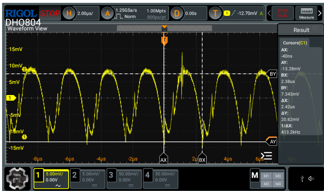
Figure 1.7: Output voltage waveform, V_{IN} = 50\text{ V} , V_{OUT} = 12\text{ V} , no load
