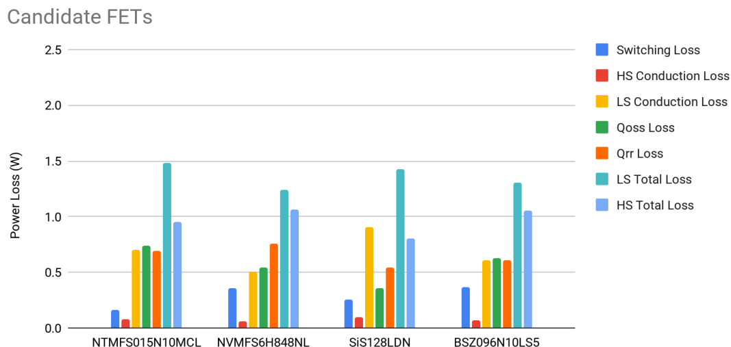
Figure 4.4: Power loss breakdown of some candidate MOSFETs.
