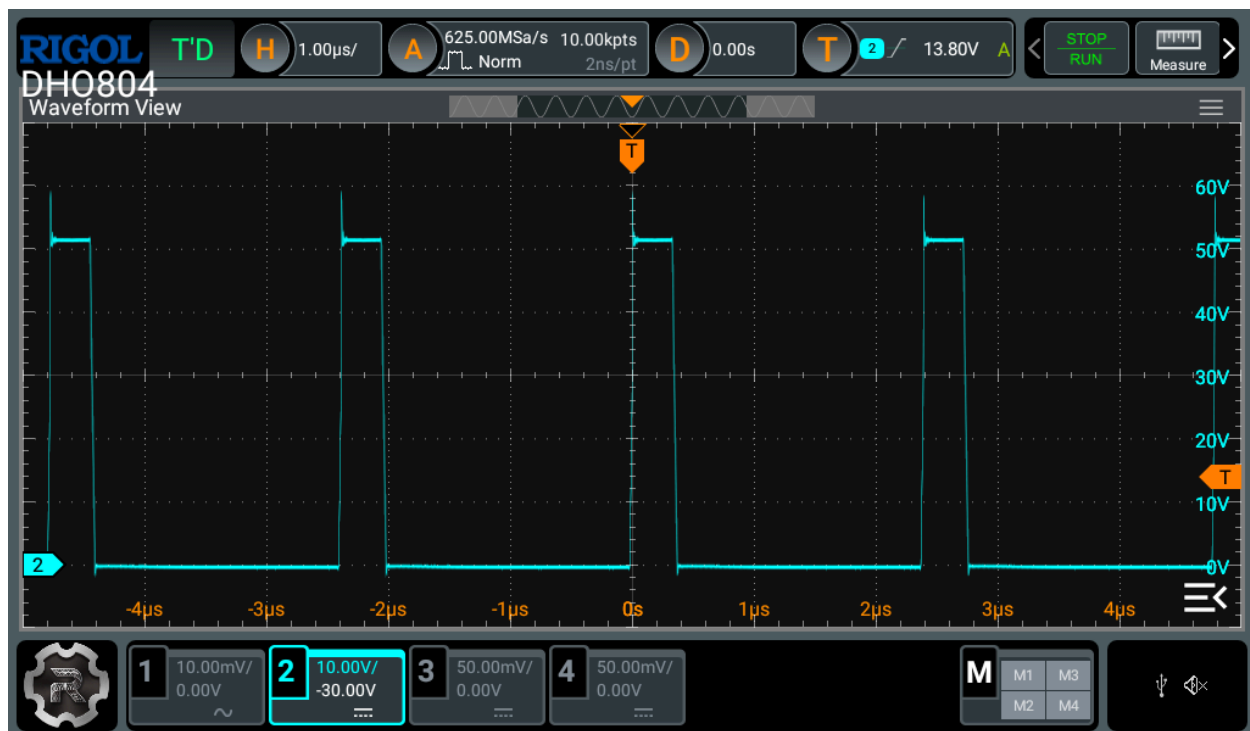
Figure 1.9: Switch-node waveform, V_{IN} = 50\text{ V} , V_{OUT} = 5.1\text{ V} , no load
